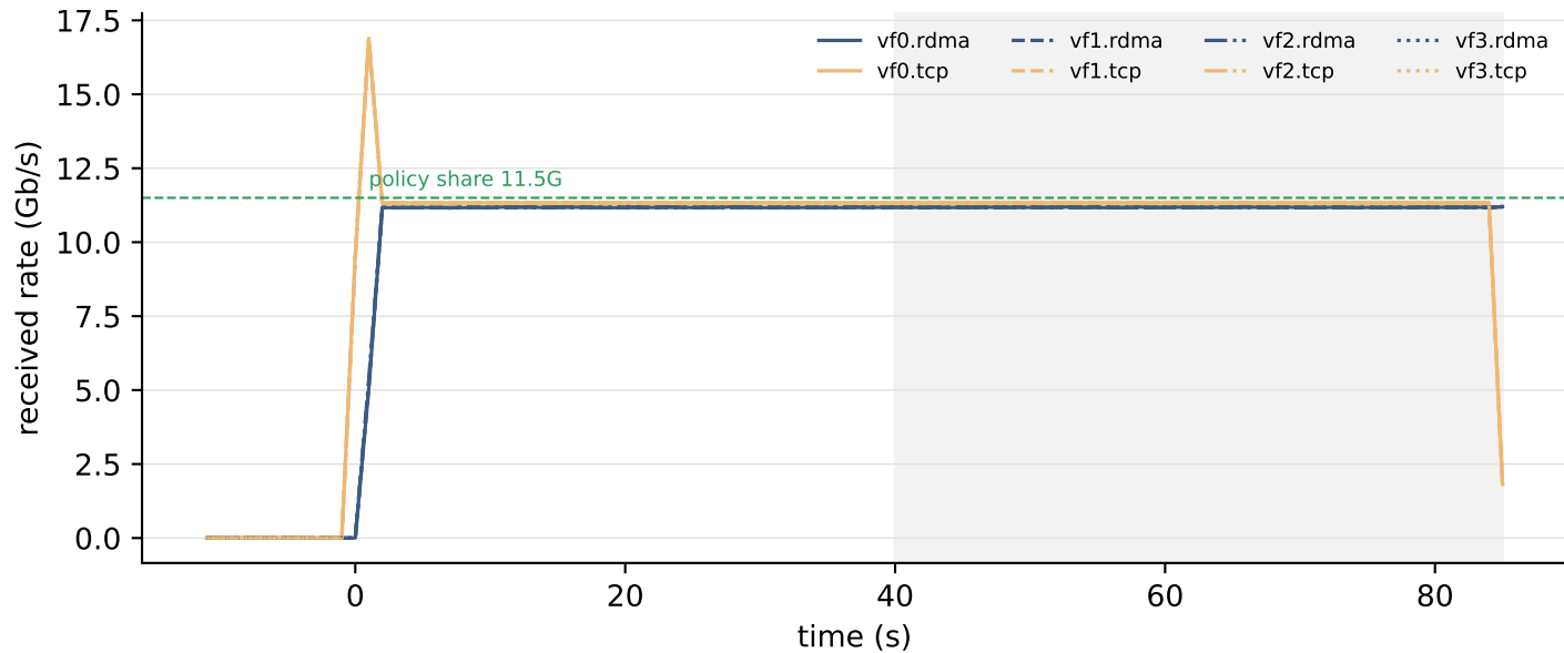
incast8 — observer, DCQCN untouched, run 4
