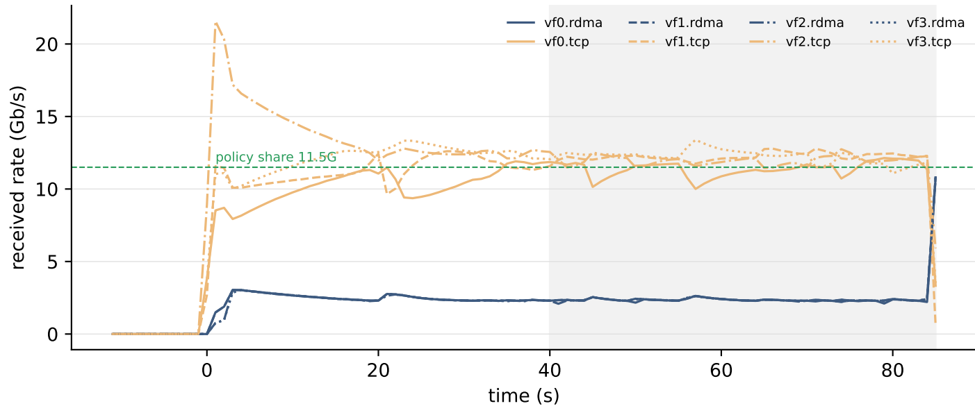
incast8 — 60G core shaper, observer on both classes
