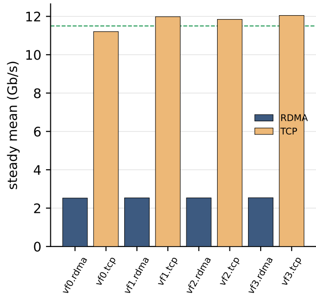
Jain=0.705 agg=57G
