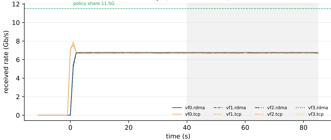
incast8 — 60G shaper, allocator told 60G, observer
