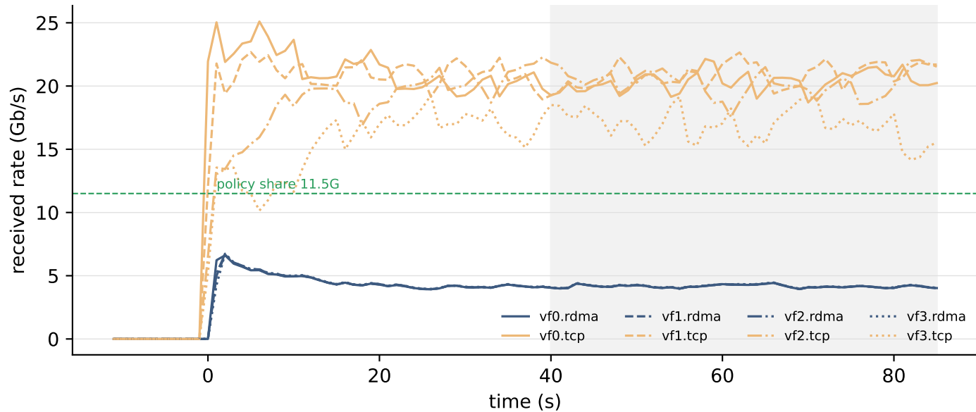
incast8, levels oversubscribed 4x — RDMA observer active branch
