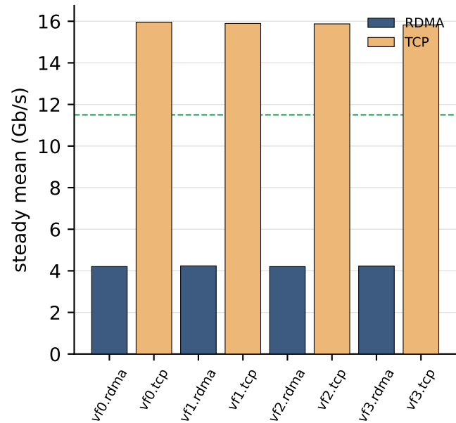
Jain=0.748 agg=80G
