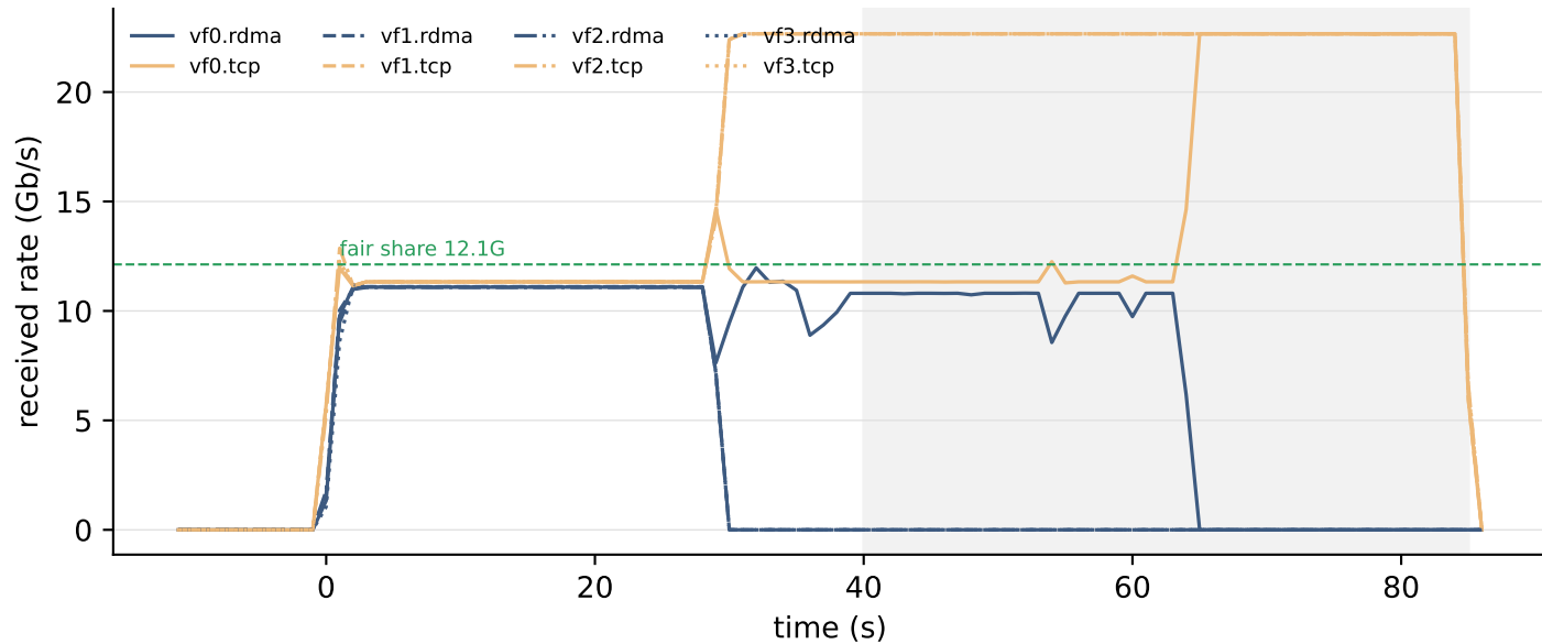
incast8 — RDMA READ (responder on sgpu01)
