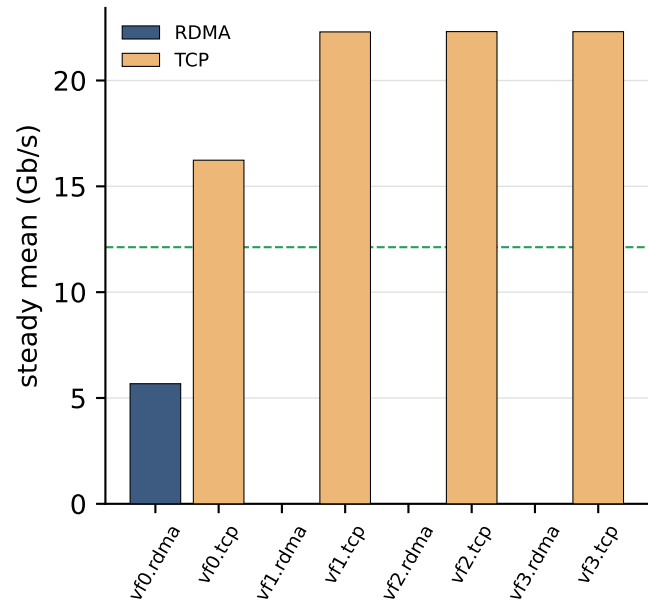
Jain=0.551 agg=89G
