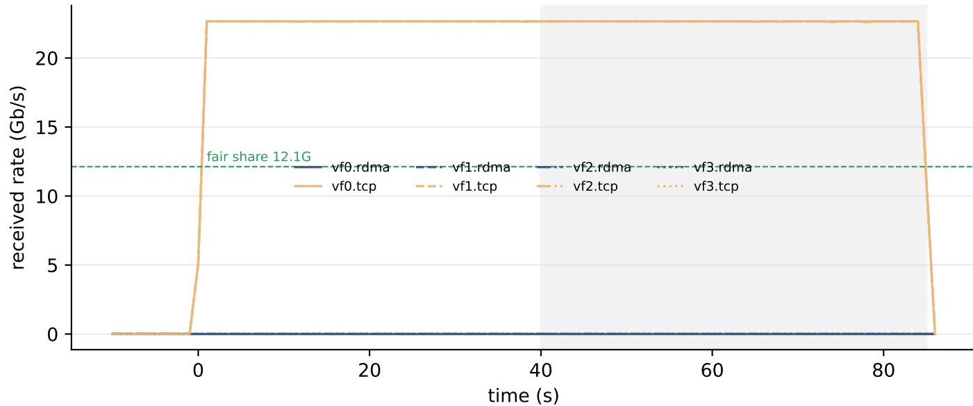
incast8 — READ, CC term = AIMD (mode 0), run 2
