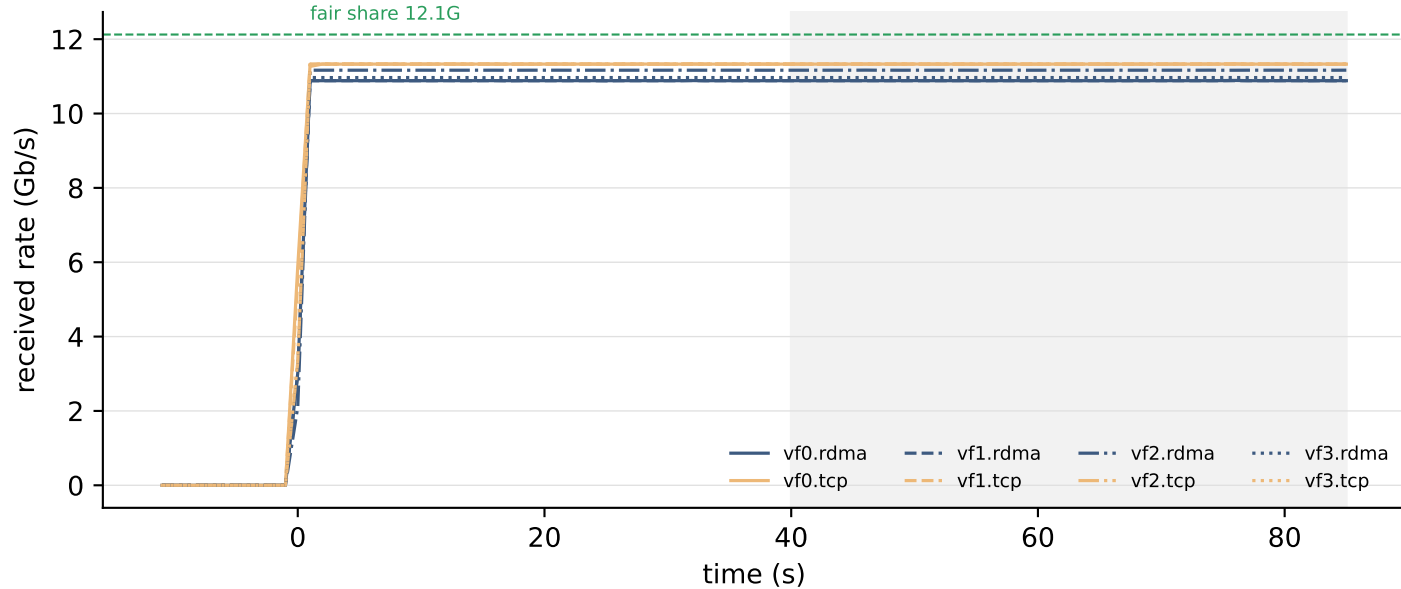
incast8 — READ, CC term = AIMD (mode 0), run 3
