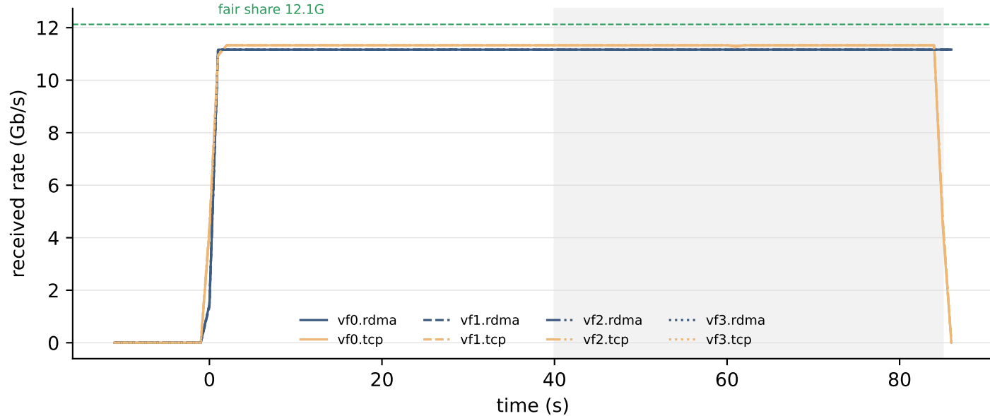
incast8 — READ, CC term = AIMD (mode 0), run 4
