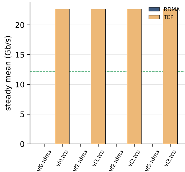
Jain=0.500 agg=91G
