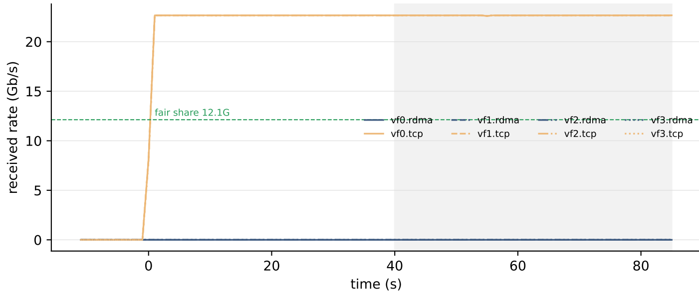
incast8 — READ, N hold 32 ms, run 1
