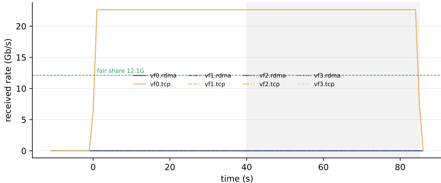
incast8 — READ, N hold 32 ms, run 2
