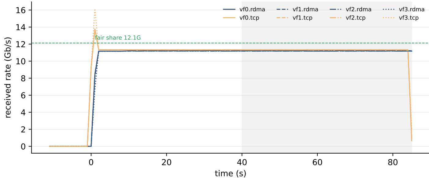
incast8 — WRITE, CC term = AIMD (mode 0), run 1
