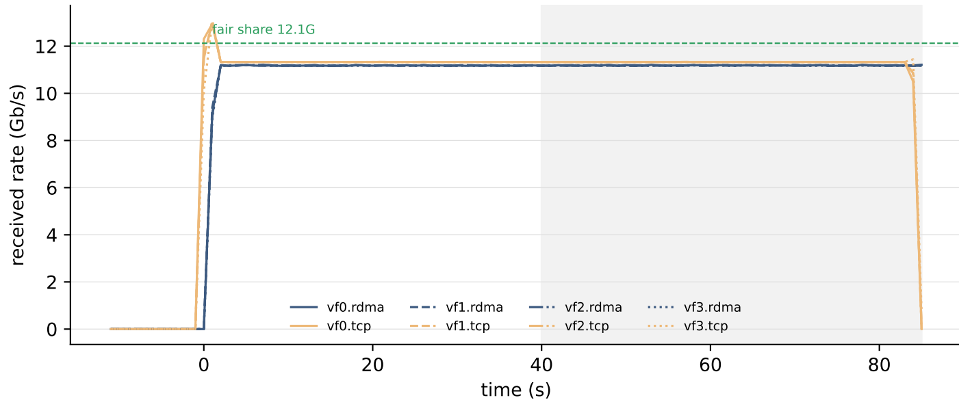
incast8 — WRITE, CC term = AIMD (mode 0), run 2
