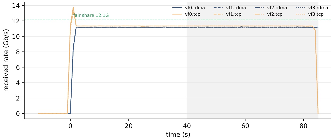
incast8 — WRITE, CC term = AIMD (mode 0), run 4
