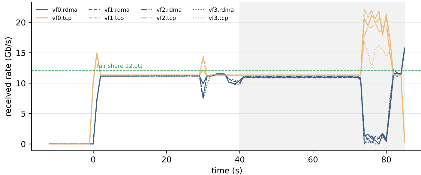
incast8 — RDMA WRITE (control)
