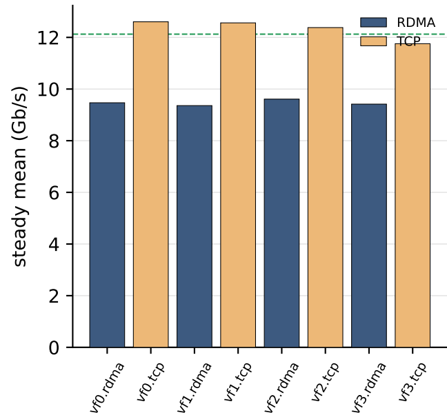
Jain=0.983 agg=87G
