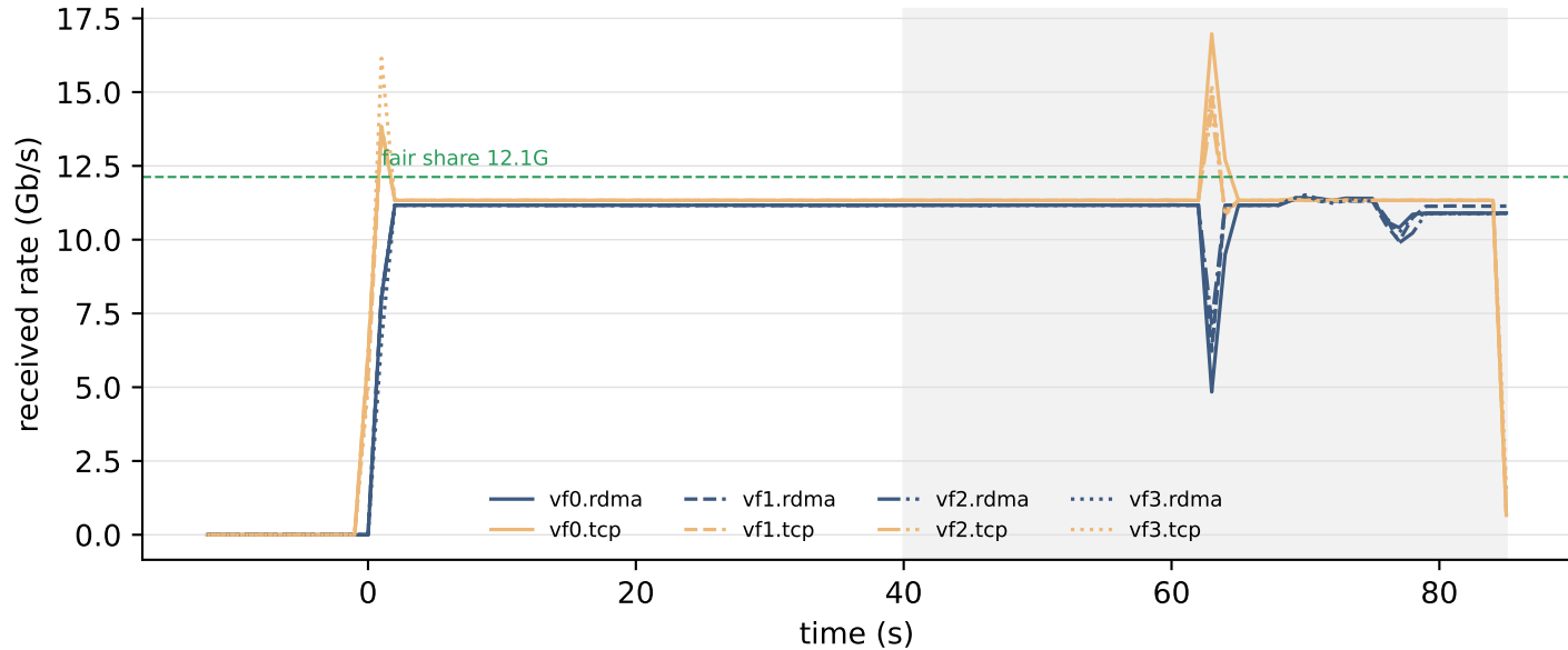
incast8 — WRITE, N hold 32 ms, run 1
