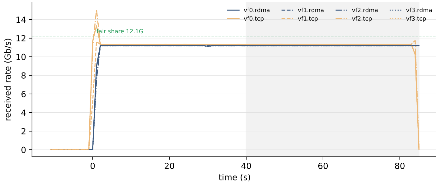
incast8 — WRITE, N hold 32 ms, run 2
