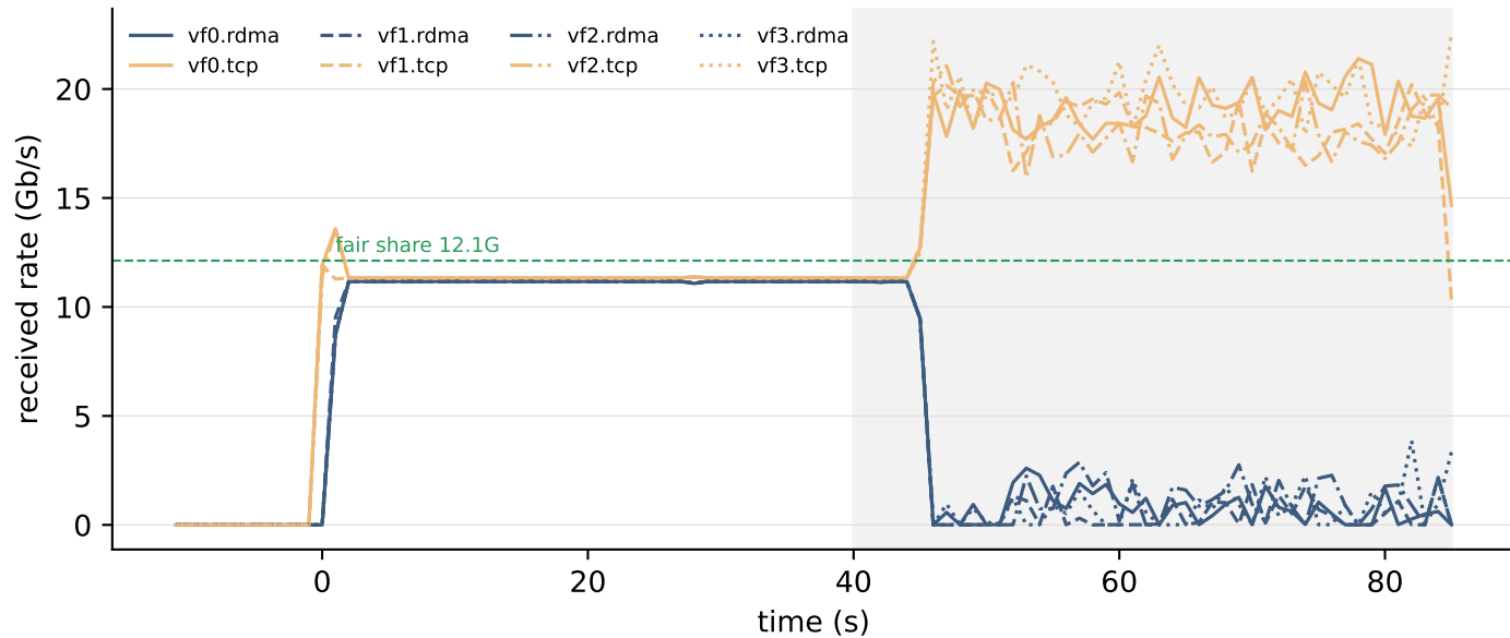
incast8 — WRITE, N hold 32 ms, run 3
