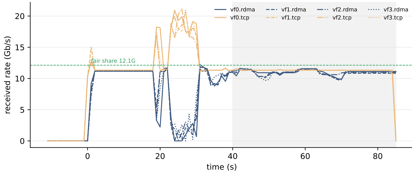
incast8 — WRITE, N hold 32 ms, run 4
