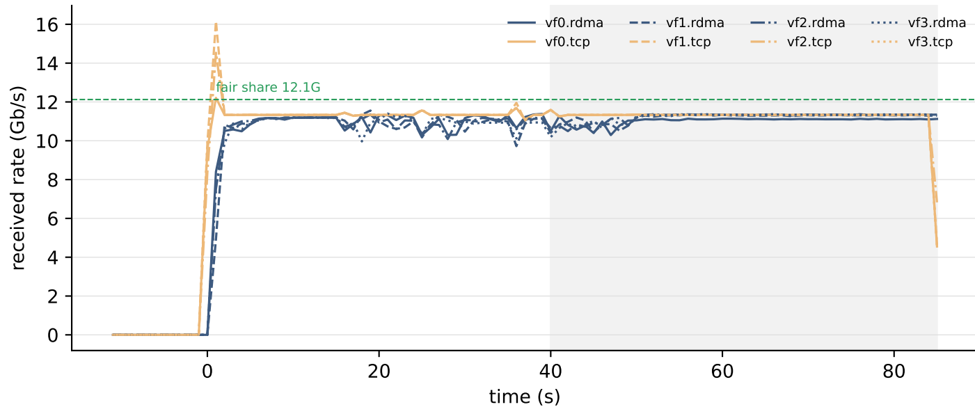
incast8 — WRITE, shallow ECN (100K/400K) run 1
