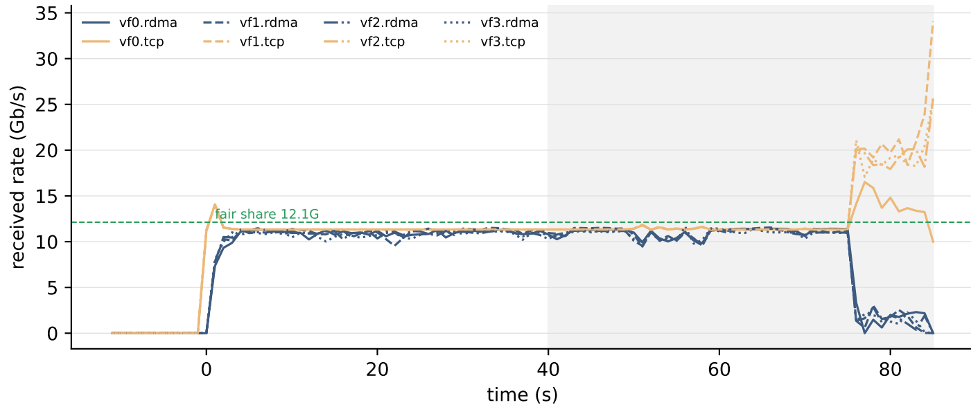
incast8 — WRITE, shallow ECN (100K/400K) run 3
