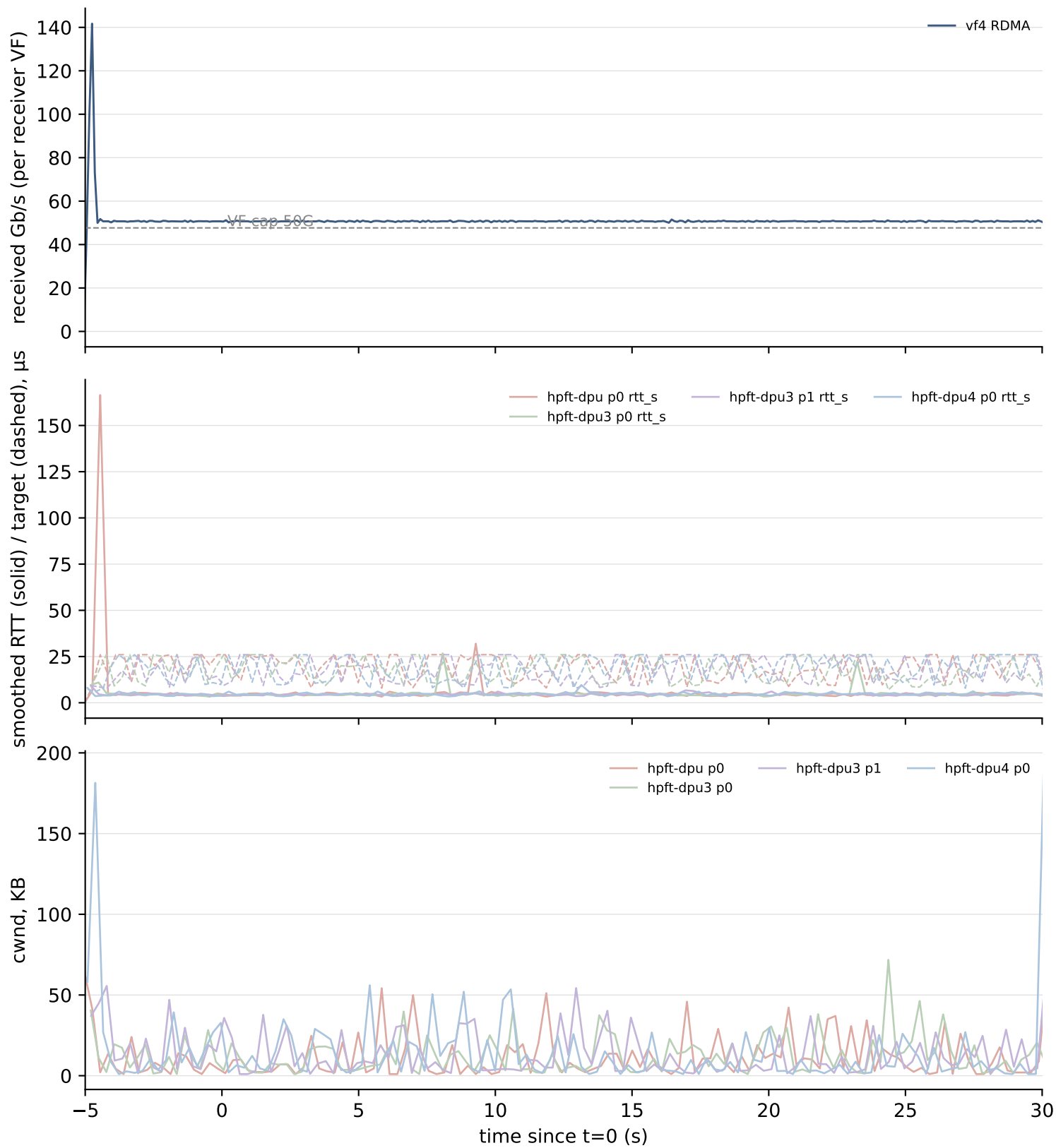
Swift on the HPFT executor - incast4_v1
