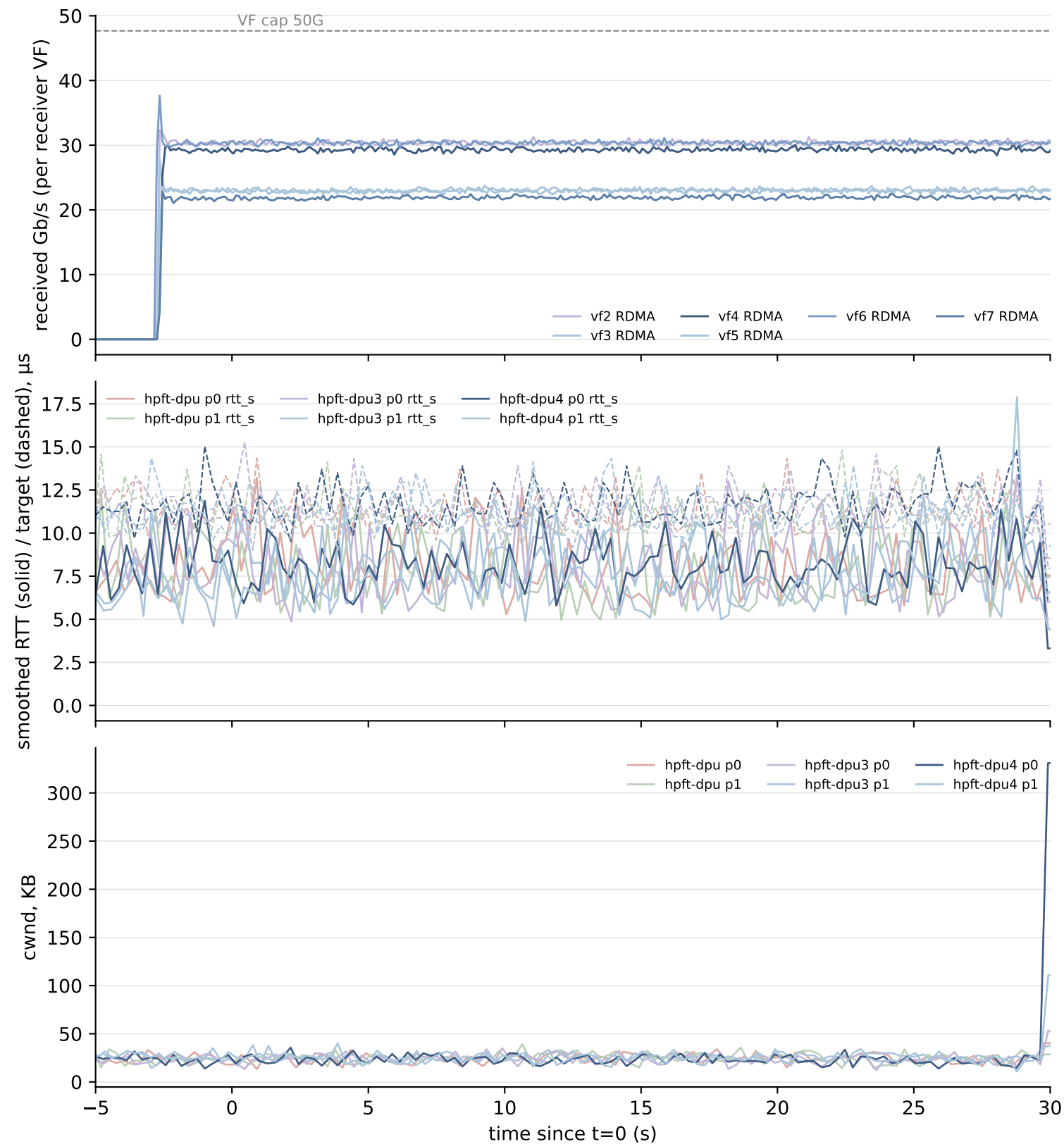
Swift on the HPFT executor - port6_swift_v1
