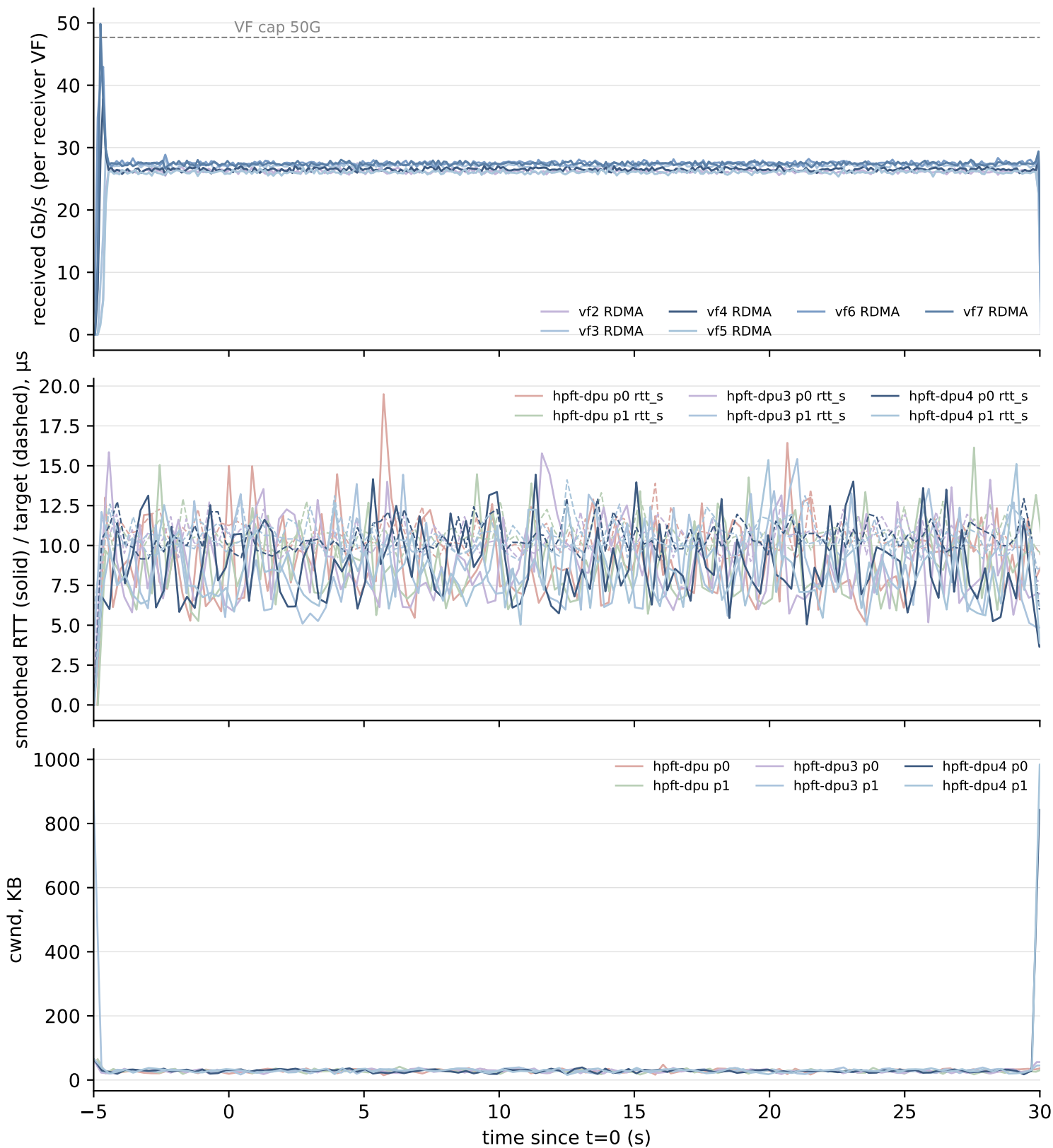
Swift on the HPFT executor - port6_swift_v2
