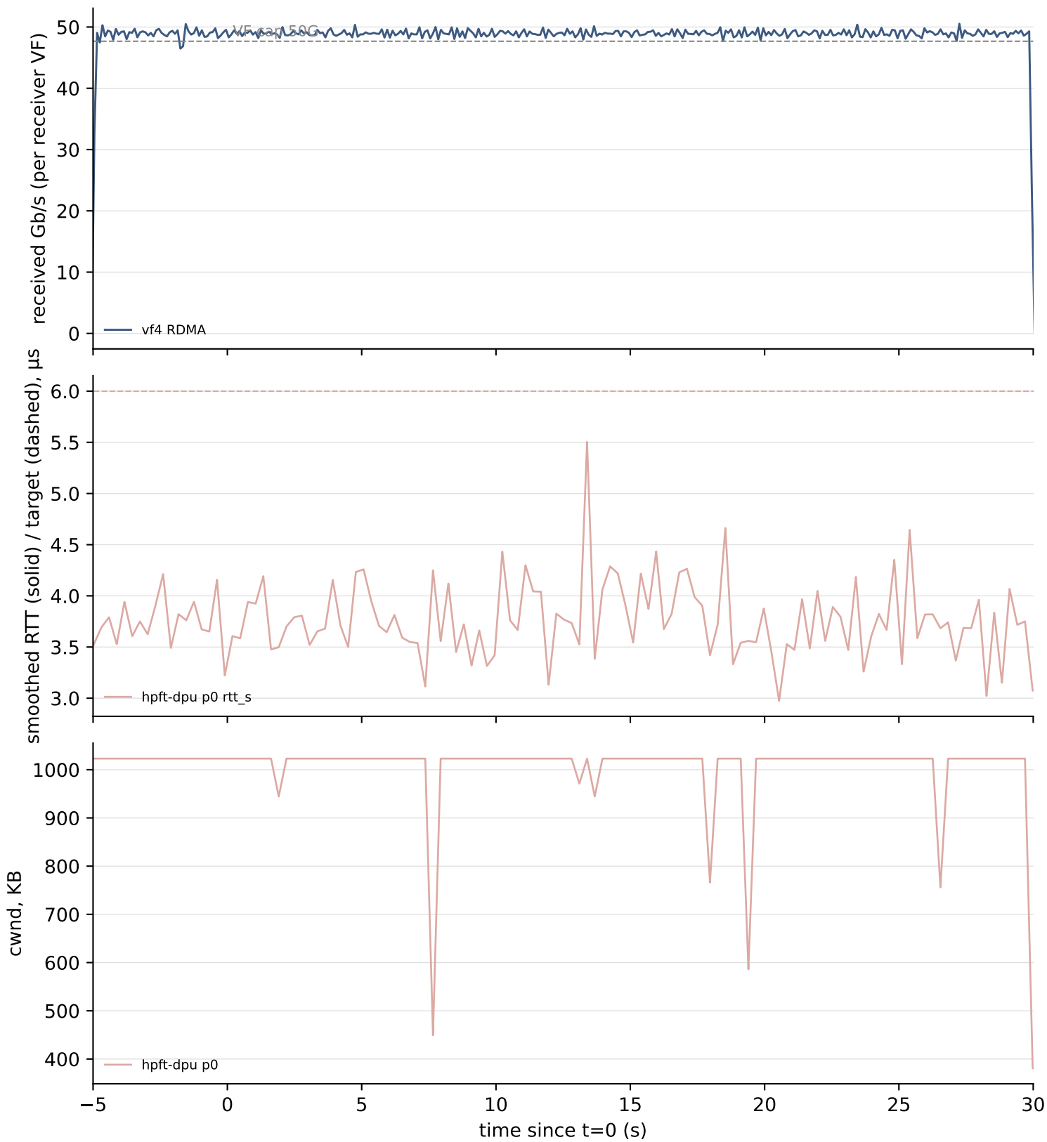
Swift on the HPFT executor - solo_v1
