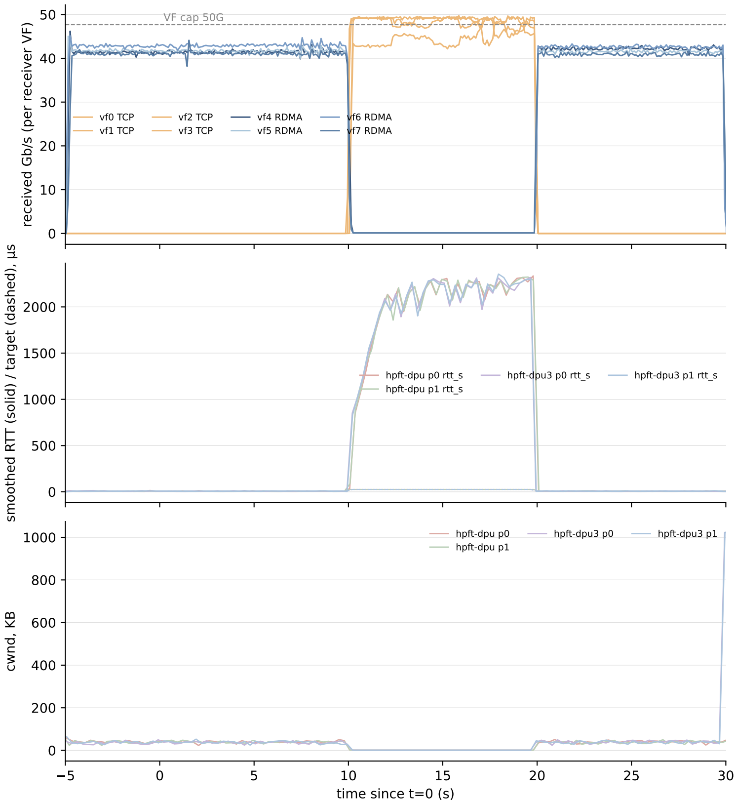
Swift on the HPFT executor - tcpmix_v1
