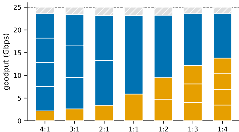
Per-class queues 60/40, RDMA-GBN
