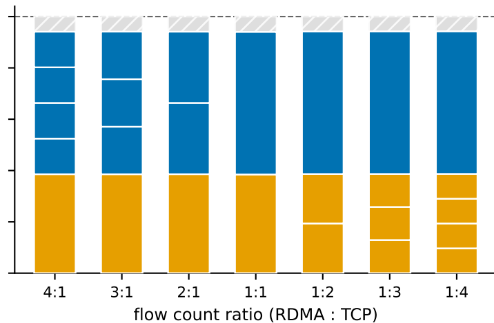
Per-class queues 60/40, RDMA-SR
