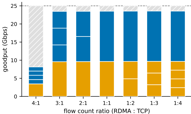
Per-class queues 60/40, RDMA-GBN
