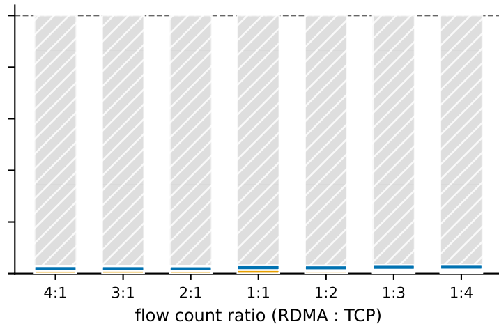
Shared queue (no ECN), RDMA-SR
