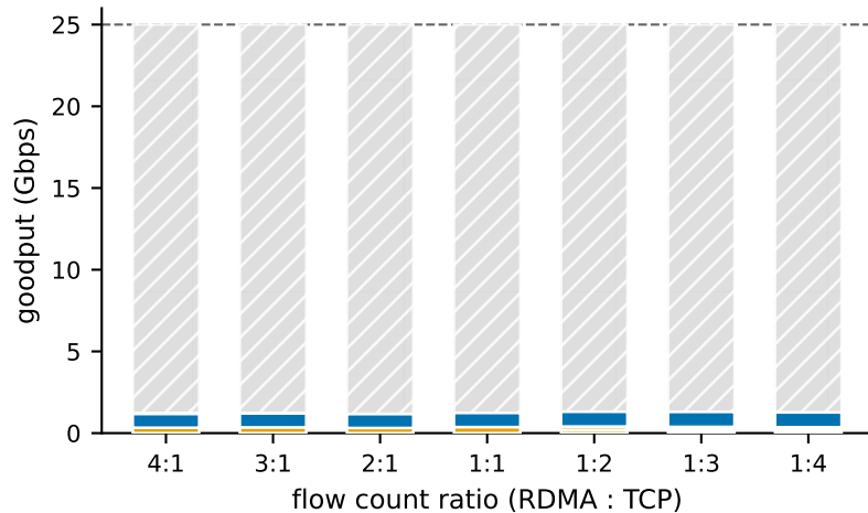
Shared queue (no ECN), RDMA-GBN
