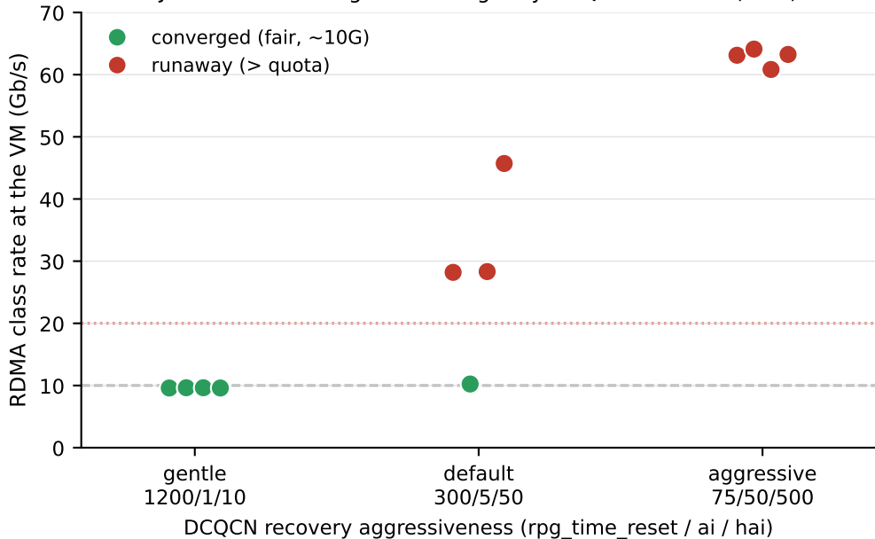
Jakiro fairness hinges on how gently DCQCN recovers (GBN)
