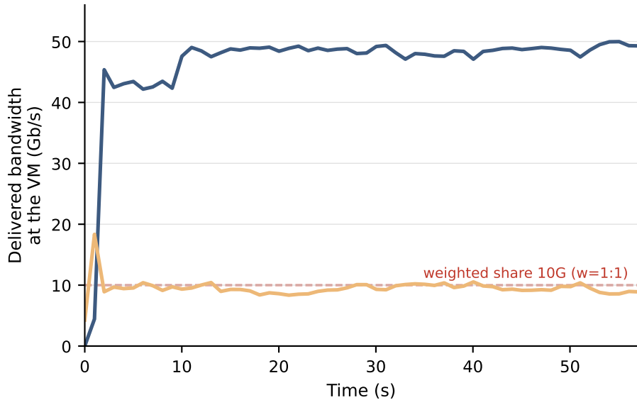
(a) Go-Back-N (RDMA repeats: 28 / 10 / 45G — bistable)
