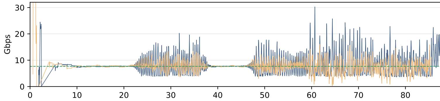
vq: hold 50 ms, eps 5%, D_r 60 ms
