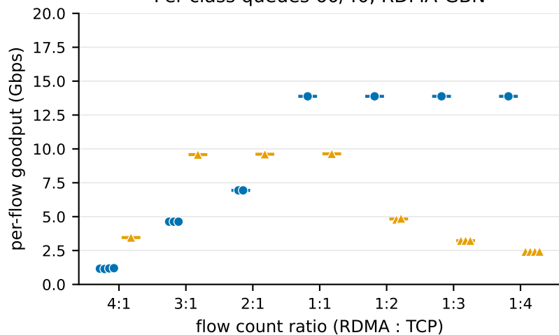
Per-class queues 60/40, RDMA-GBN
