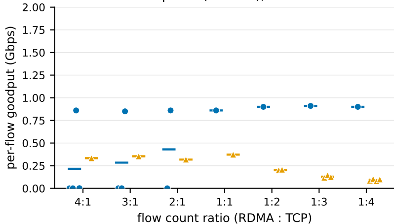
Shared queue (no ECN), RDMA-GBN
