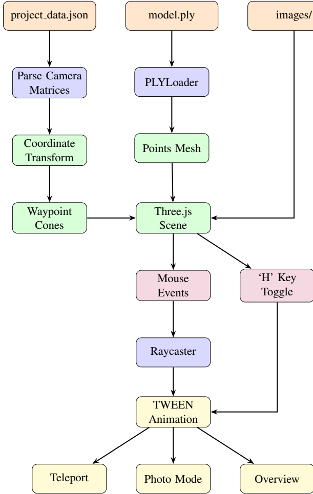
Figure 4: Virtual tour viewer architecture. SfM outputs (JSON camera data and PLY point cloud) are loaded and transformed to Three.js coordinates. User interactions trigger raycasting or keyboard handlers that animate the camera via TWEEN.js.
