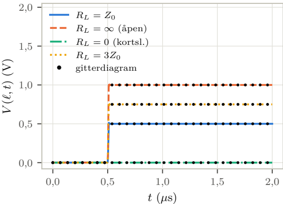
(a) Tapsfri linje, R_s = Z_0
