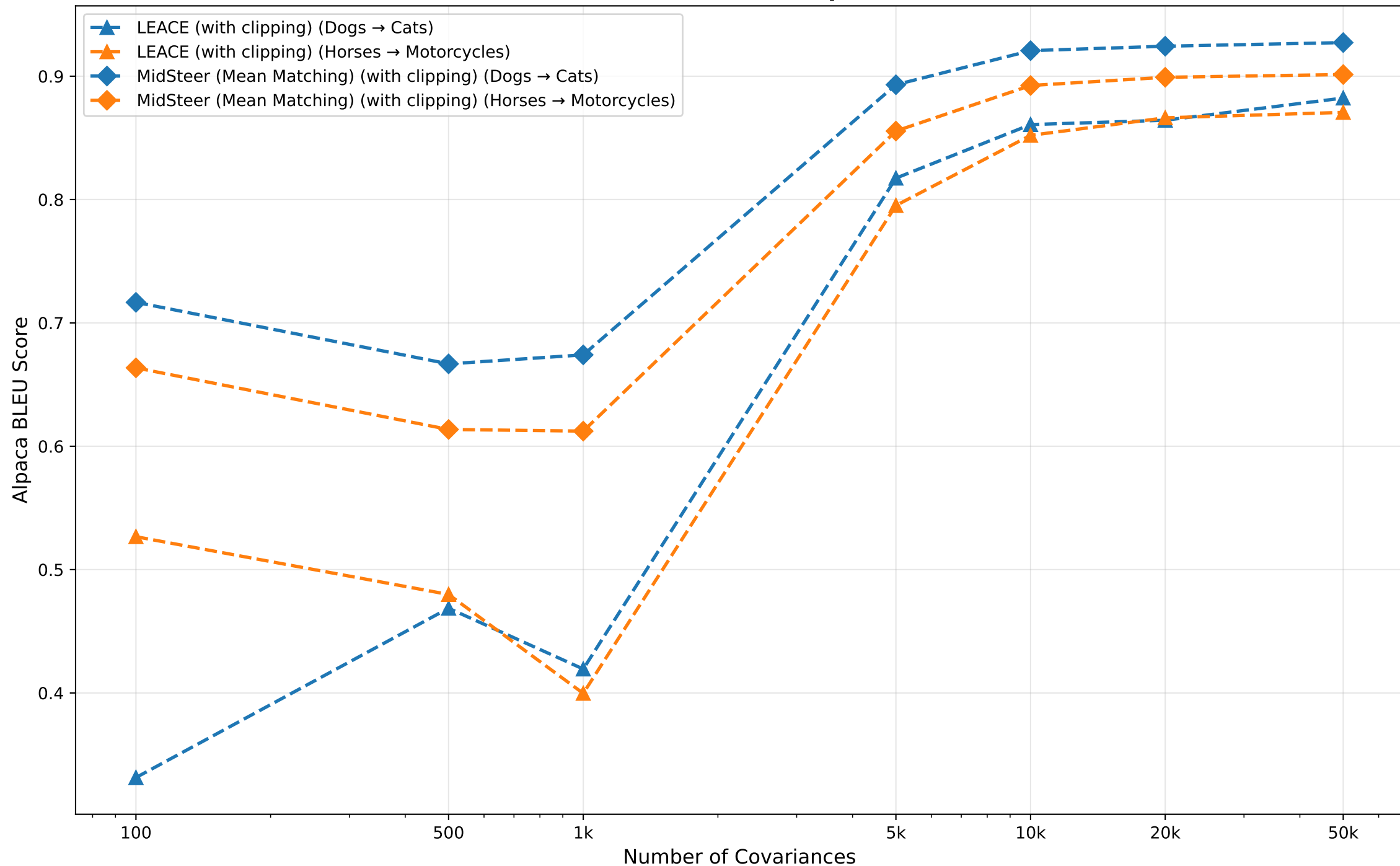
Alpaca BLEU Score vs Number of Covariances Combined Tasks Comparison
