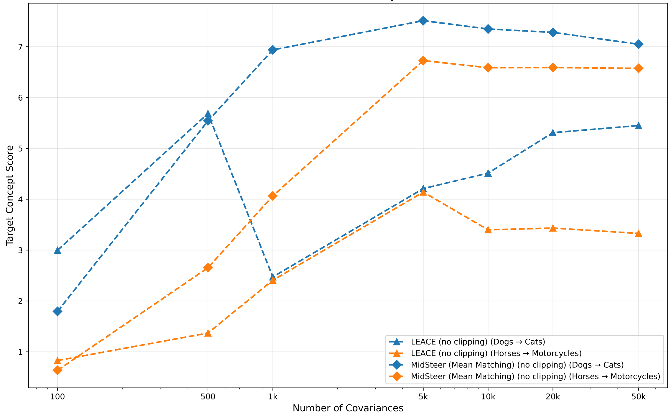
Target Concept Score vs Number of Covariances Combined Tasks Comparison
