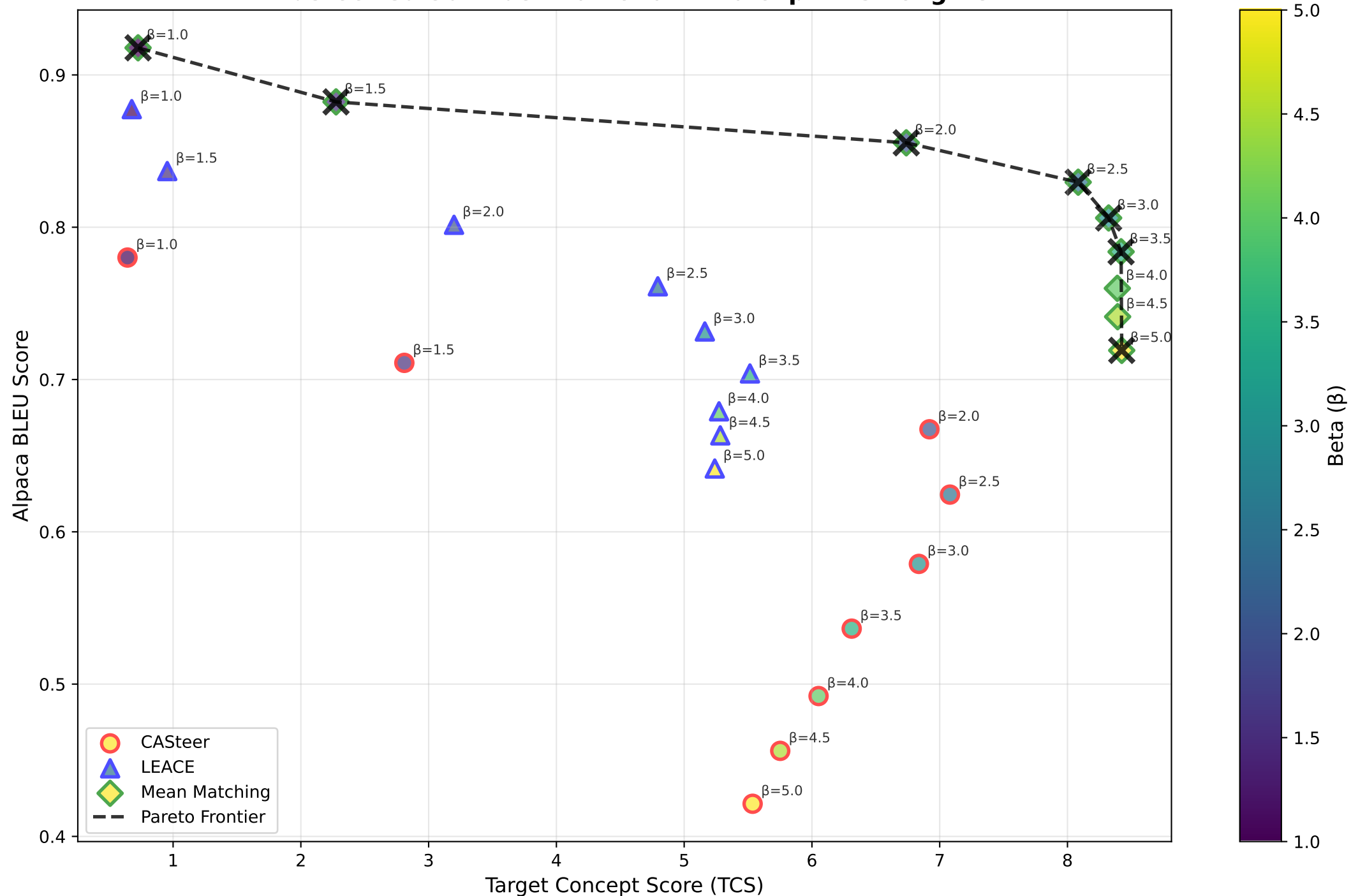
Pareto Frontier: Horses → Motorcycles Midsteer Sa 50K Last No Renorm No Clip All Strengths
