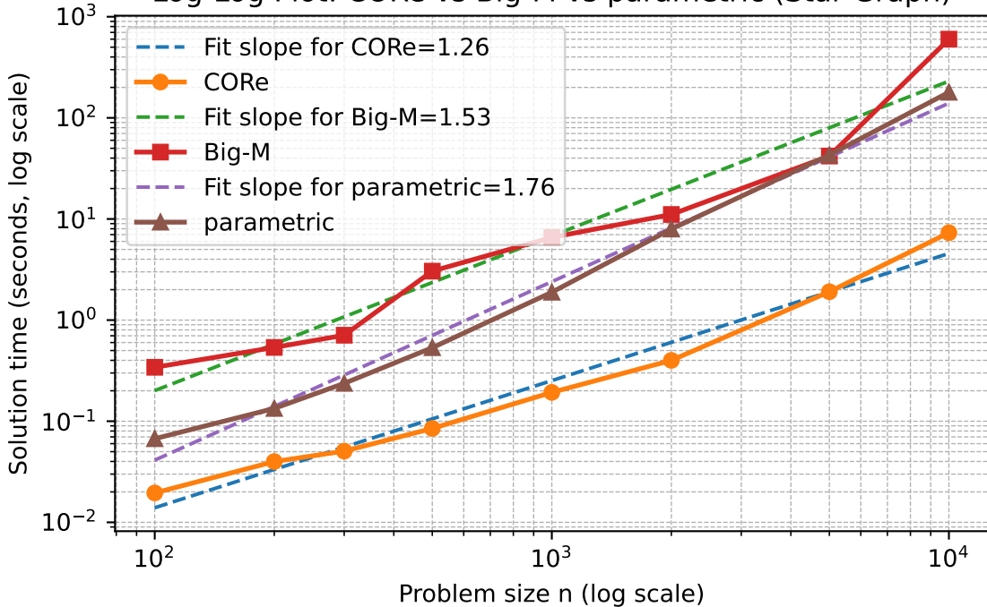
Log-Log Plot: CORE vs Big-M vs parametric (Star Graph)
