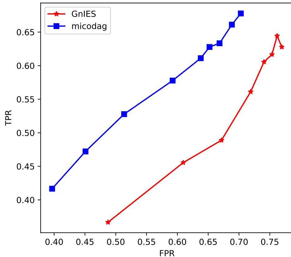
Semi-synthetic data from fitted consensus network
