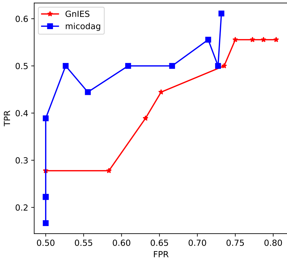
Real data (Sachs et al. 2005)
