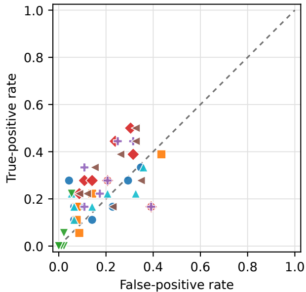
Directed edges
