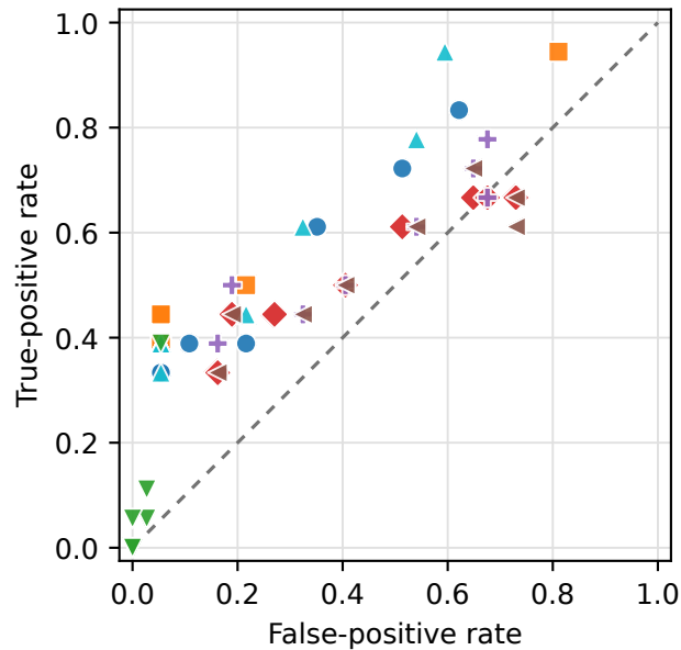
Skeleton edges
