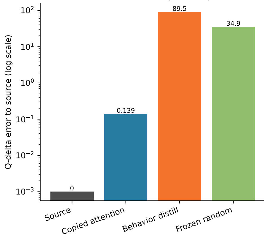
Counterfactual geometry
