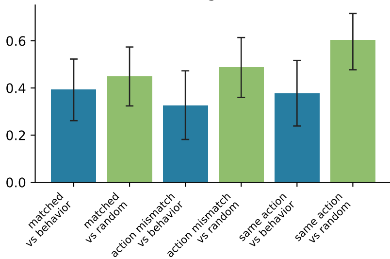
Action agreement
