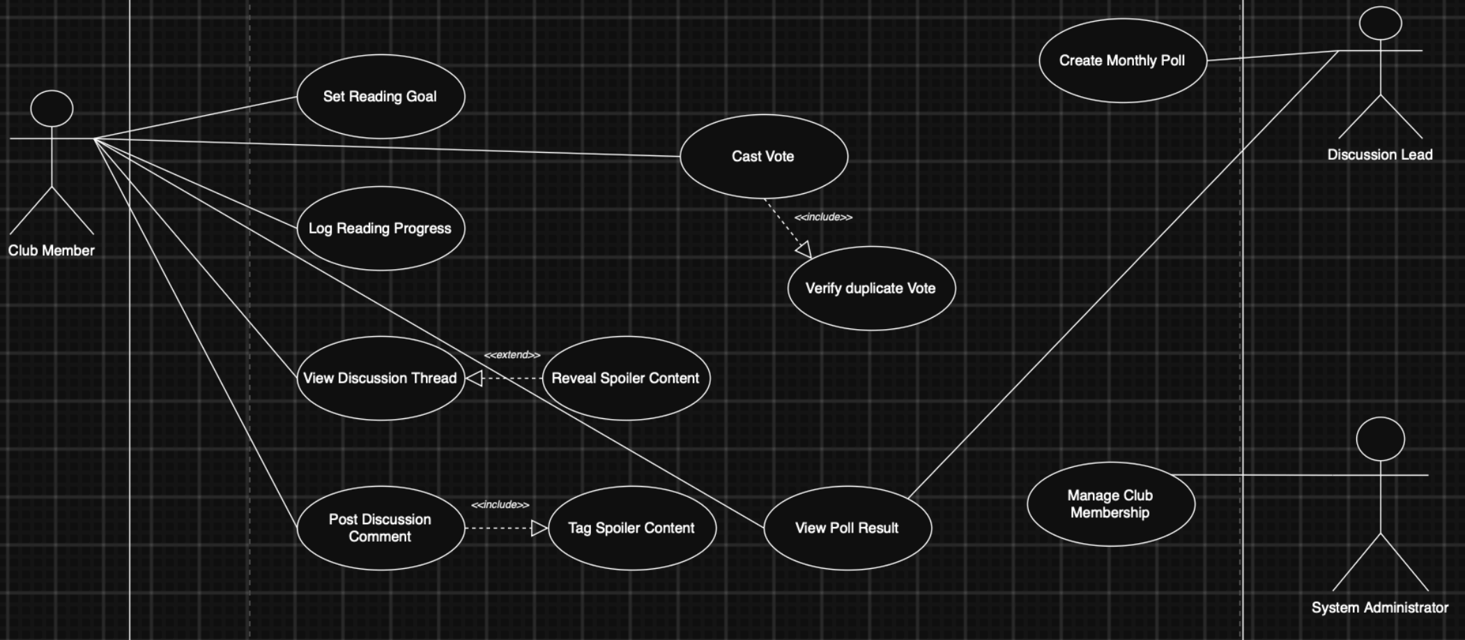
Book Club Reading Challenge & Discussion Portal UML Use-Case Diagram
