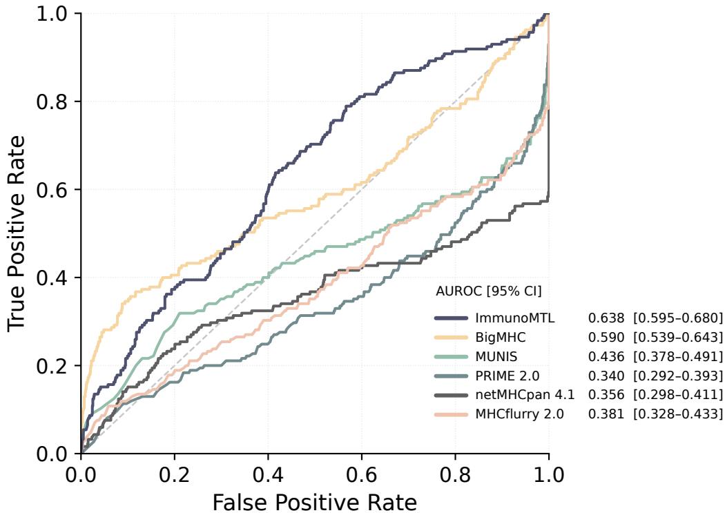
ROC — ZeroShot-1
