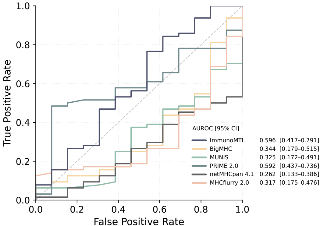
ROC — ZeroShot-2
