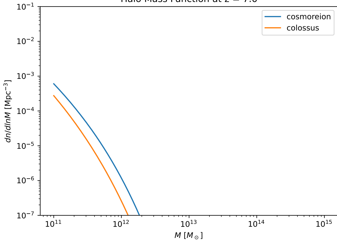
Halo Mass Function at z = 7.0
