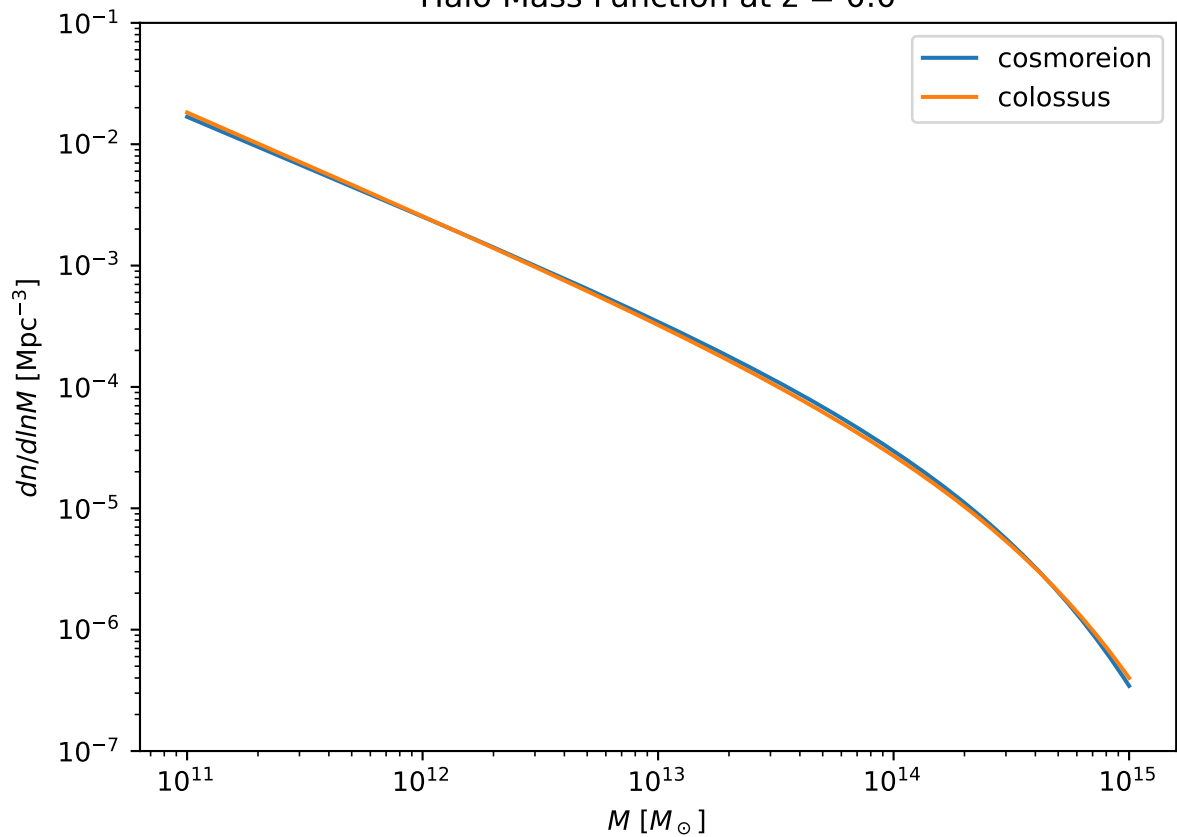
Halo Mass Function at z = 0.0
