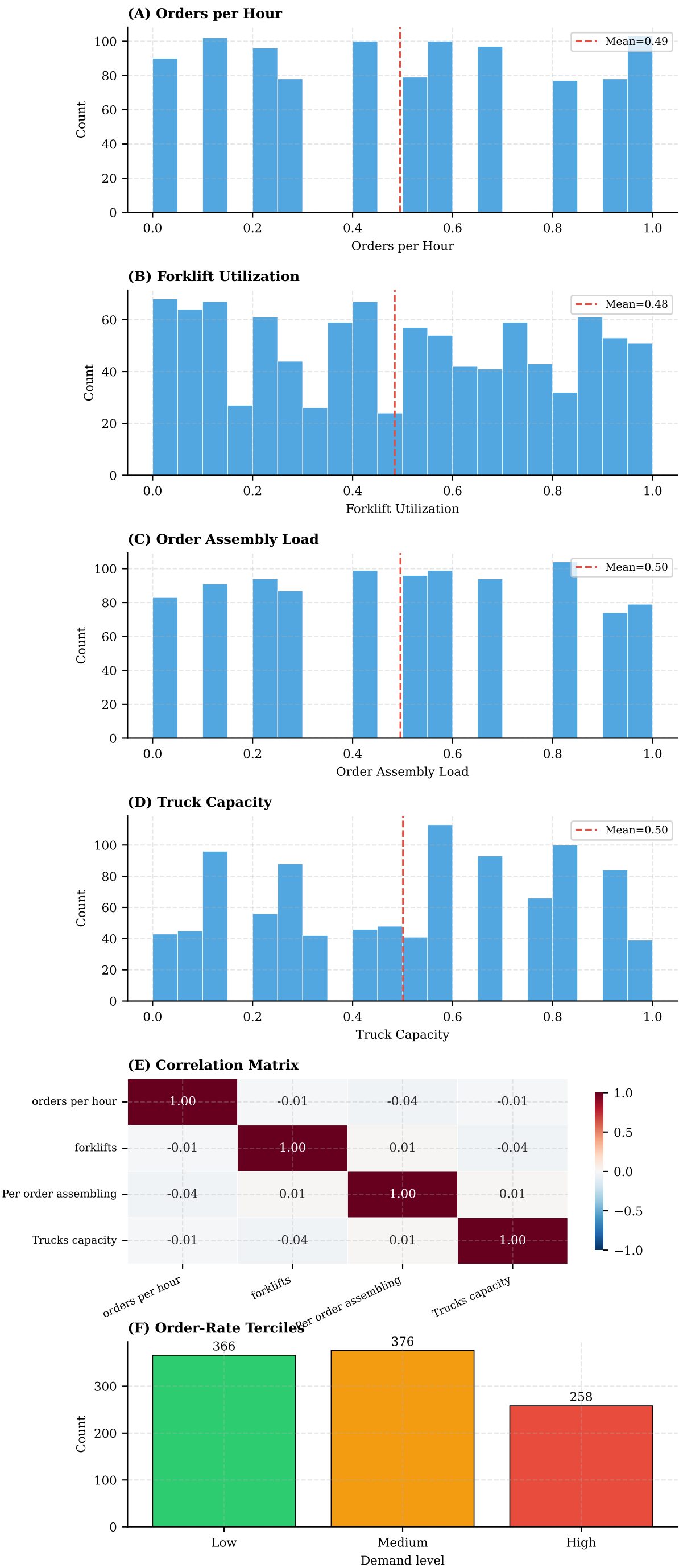
Fig. 1: Warehouse Operation Dataset (EDA)
