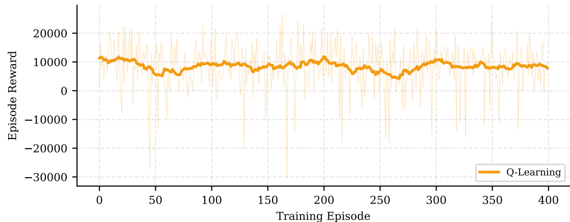
Fig. 3: Training Convergence Curves
